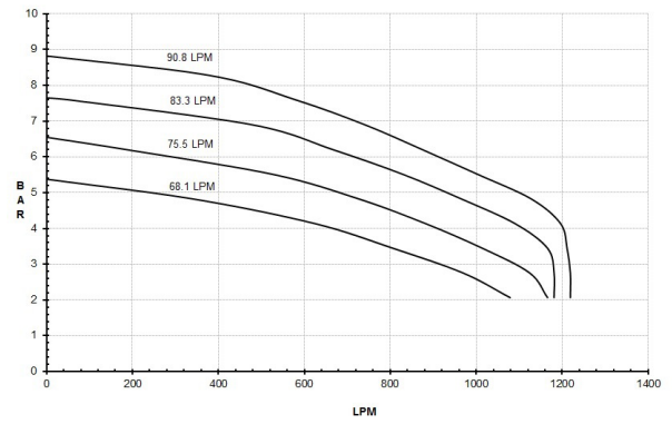
9306C-HM3C-3U & 9306S-HM3C-3U METRIC
