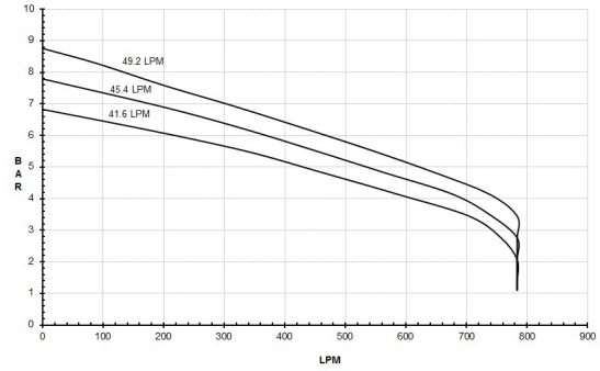
9306C-HM1C & 9306S-HM1C METRIC 9306C-HM1C-U & 9306S-HM1C-U
